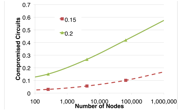
Figure 10: Estimated fraction of complete compromises for \ell = 3, \rho = 5 and f \in \{0.15, 0.2\}
