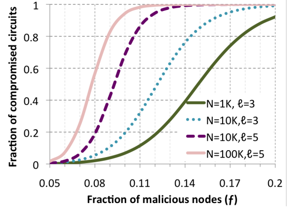
Figure 4: Overlay circuit extension: Fraction of circuits compromised as a function of fraction of compromised nodes, for varying network size ( N ) and circuit length ( \ell ), assuming Chord-style routing.
