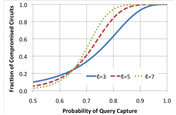
Figure 3: Fraction of circuits compromised as a function of probability of query capture, given f = 0.1 .
