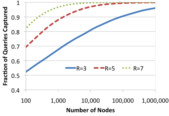
Figure 6: Results of simulated attack on Salsa with malicious fraction f = 0.1 , where conflicting redundant lookups are resolved to the closest node.
