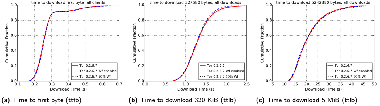
Fig. 8. Network performance under light load (796 relays, 1125 web clients with 30 bulk clients, 75 perf clients for each of 50KiB, 1MiB and 5MiB file size performing an average throughput of \approx 120 MiB/s altogether). Comparison of Waterfilling fully used on all clients versus Tor’s ABWRS used on all clients versus mix 50% of clients doing Waterfilling and 50% of clients doing Tor’s ABWRS – The topology generated is scaled down from the first consensus from May 28, 2016. Graphs are plotted until percentile 0.99.
