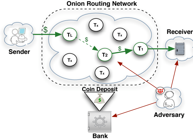
Fig. 1. The PAR architecture combines an onion routing anonymity network (Tor) with a payment scheme. Each node T_1, T_2, T_3, \dots, T_L , where L is the path length, in the path from the sender to the receiver receives payment in coins for its service.
