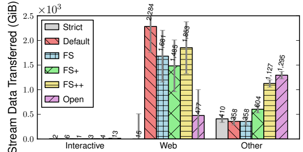
(c) Counts of data transferred on connections exiting Tor
