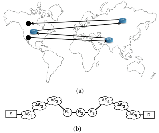
Fig. 1. (a) Random relay selection can inflate end-to-end latencies due to circuitous routing, and (b) an example in which an AS (AS2) can subvert the client's anonymity by correlating traffic across the entry and exit segments.
