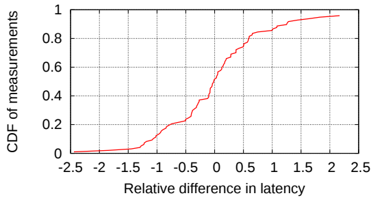
Fig. 15. Variation across time of latencies on paths spanning similar end-to-end geographical distances.
