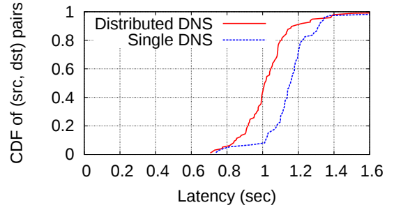
Fig. 7. Lower latencies obtained with WSP when accounting for distributed destinations.
