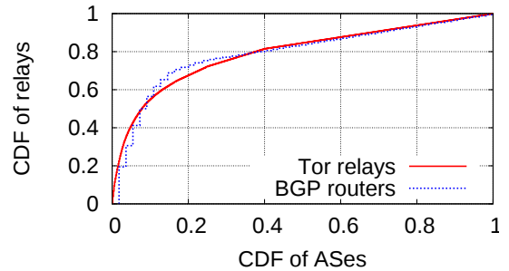
Fig. 3. Distribution of relays across ASes in PL-BGP-Rand and PL-Tor-Web datasets.
