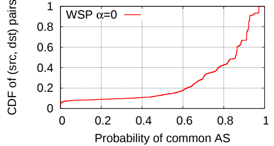
Fig. 12. The probability of existence of snooping ASes across (src, dst) pairs in the PL-BGP-Rand dataset.
