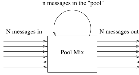
Figure 2.1: The pool mix
