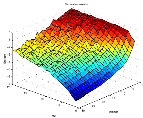
(a) Exponential mix simulation results
