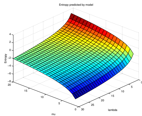
(b) Metric predictions for exponential mix
