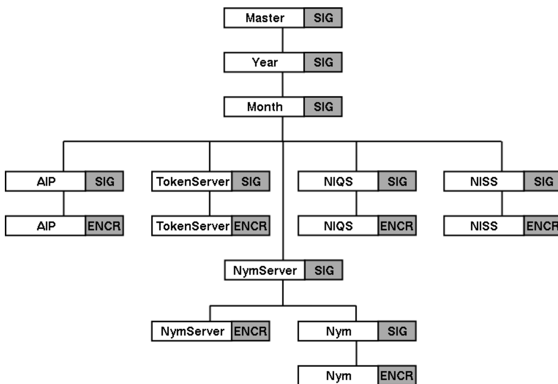
Figure 6: Key Hierarchy
