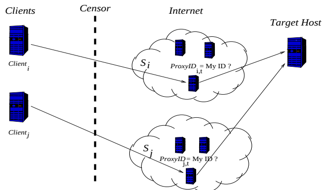
Fig. 3. In keyspace hopping, clients and proxies agree on which proxy forwards which client's request. Each client discovers a unique set of proxies.
