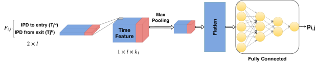
Figure 14: The network architecture of DeepCorr to detect stepping stone attacks
