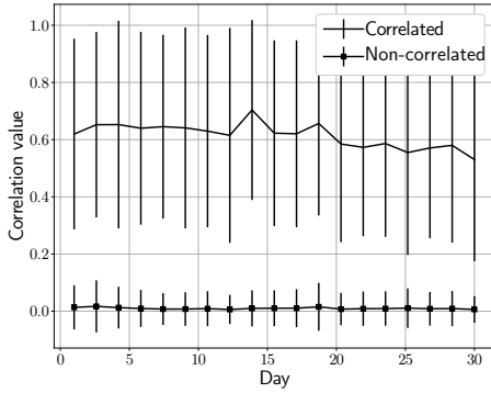
Figure 6: DeepCorr’s correlation values for associated and non-associated flows for 30 consecutive days without re-training. The performance only starts to drop after about three weeks.
