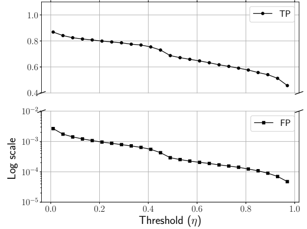
Figure 4: True positive and false positive error rates of DeepCorr in detecting correlated pairs of ingress and egress Tor flows for different detection thresholds ( \eta ). Each flow is only 300 packets.
