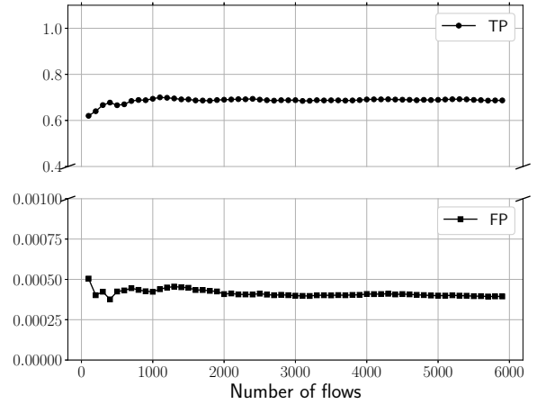
Figure 7: DeepCorr’s performance is consistent regardless of the size of the testing dataset (we use a fixed, arbitrary \eta ).
