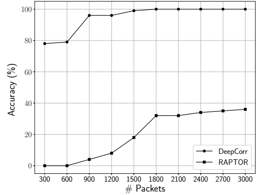
Figure 13: Comparing DeepCorr to RAPTOR in correlating short flows.
