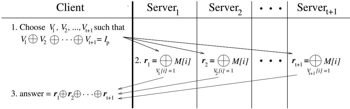
Figure 3: Bit-Vector Protocol
