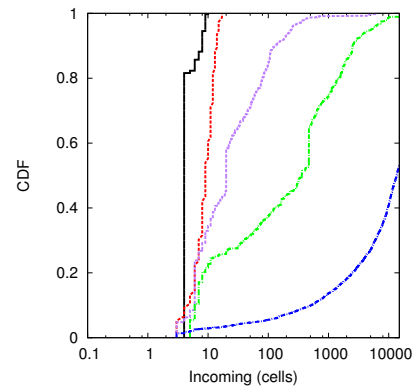
(c) Distribution of the number of incoming cells (i.e., cells sent to the client or from the server) of different Tor circuits.
