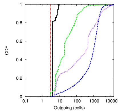
(b) Distribution of the number of outgoing cells (i.e., cells sent from the client or from the server) of different Tor circuits.
