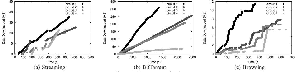
Figure 1: Downstream circuits
