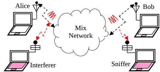
Fig. 2. Flow Marking Attack Scenario
