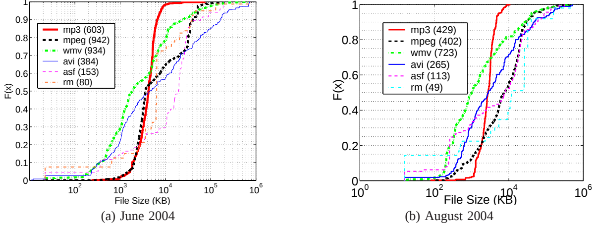
Fig. 11. Audio/Video file size distribution within KaZaA (numbers besides file types denote the number of such files within one week)
