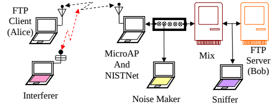
Fig. 5. Experiment Setup
