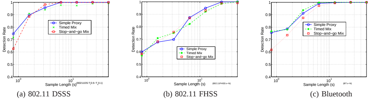
Fig. 7. Detection Rate by Flow Marking Attack
