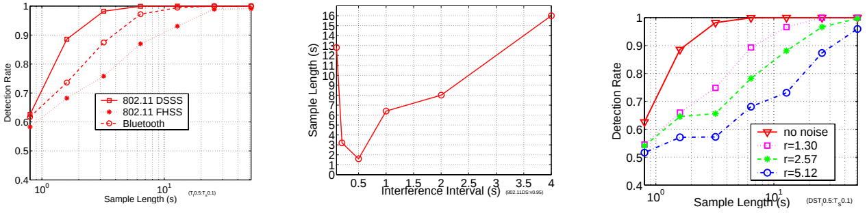
Fig. 9. Sample Length Required to Achieve Detection Rate of 95%
