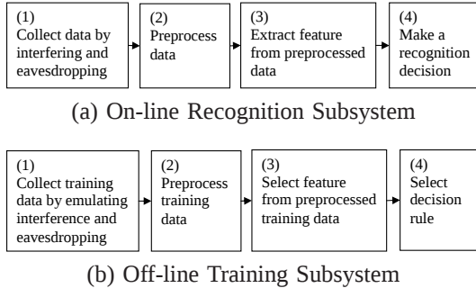
Fig. 3. Flow Marking Attack Framework
