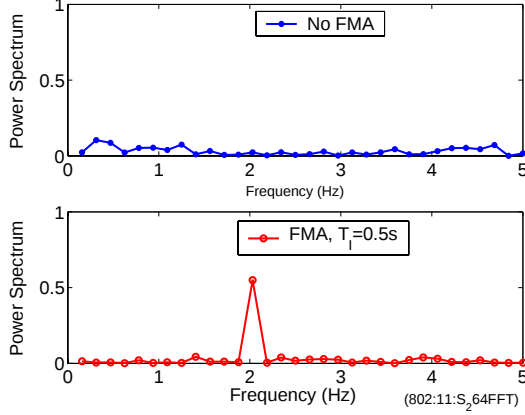
Fig. 6. Power Spectrum of 802.11 DSSS Traffic for stop-and-go mix
