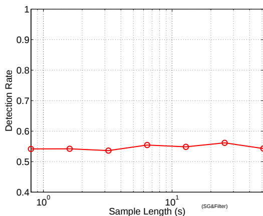
Fig. 12. Detection rate with filter-based countermeasure
