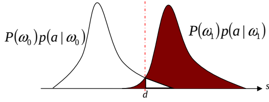
Fig. 4. Bayes Decision Rule for Flow Marking Attack
